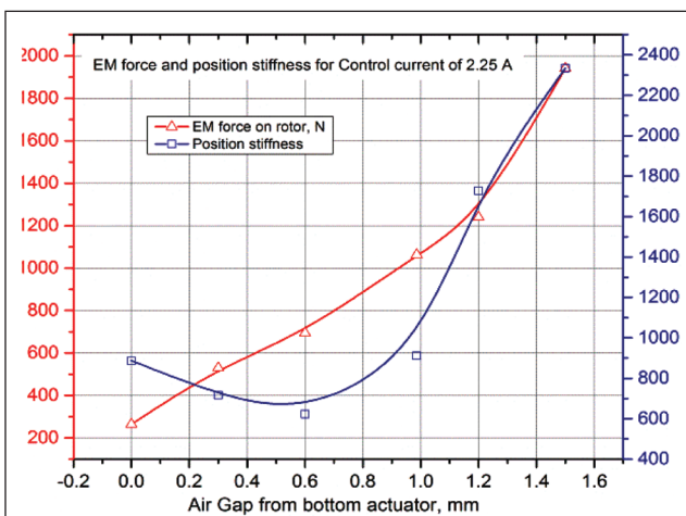
FIG. 20 EM FORCE-ROTOR POSITION AND POSITION STIFFNESS CONTROL CURRENT OF 2.25 A (REQUIRED WHEN ROTOR AT BOTTOM END)
