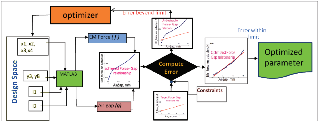
FIG. 7 PROCESS FLOW AS IMPLEMENTED IN OPTIY INTEGRATED WITH MATLAB
