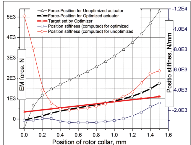
FIG. 16 COMPARISON OF OPTIMIZED AND UN OPTIMIZED ACTUATOR
